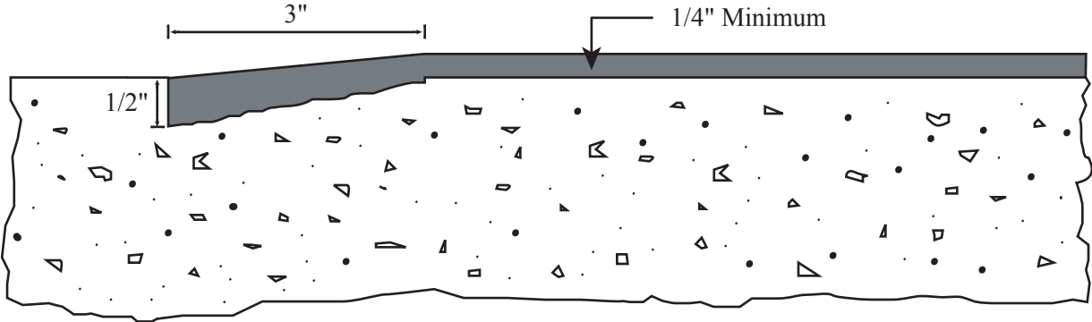
(3) Finished Chase
