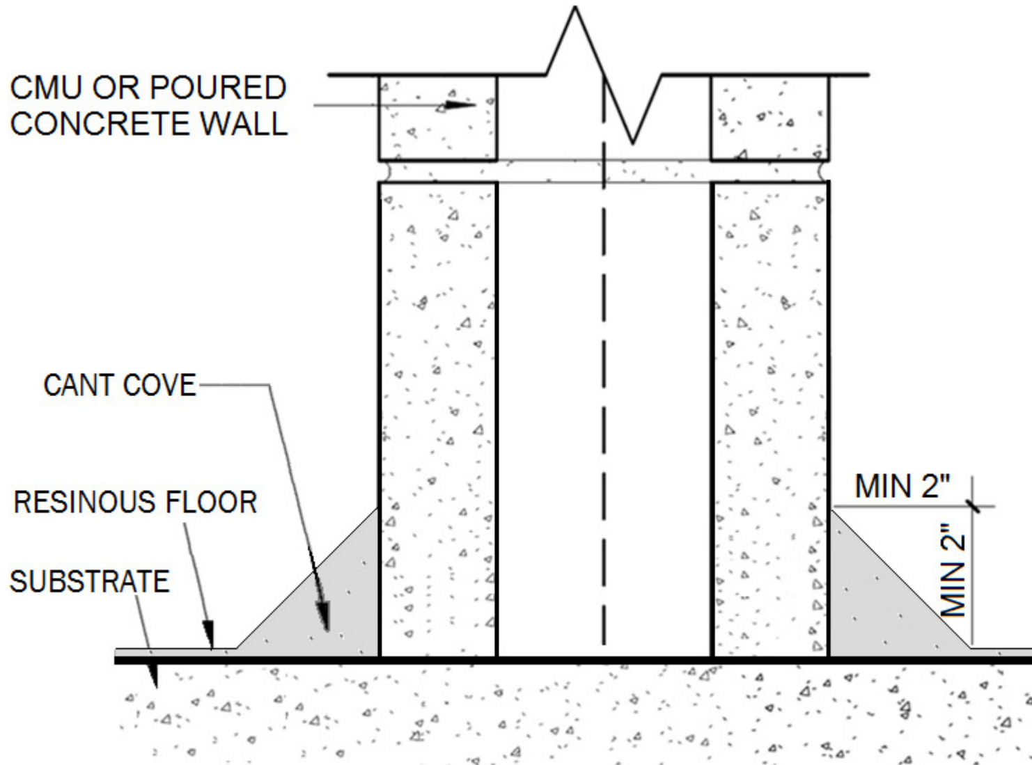
INSTALLATION DETAILS
