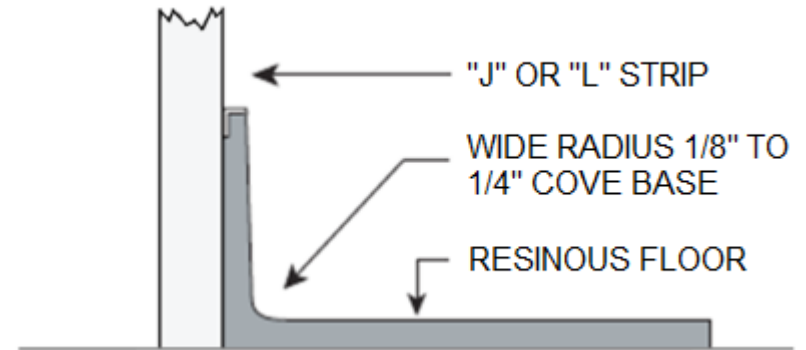
FLUSH COVE W/ J or L STRIP
